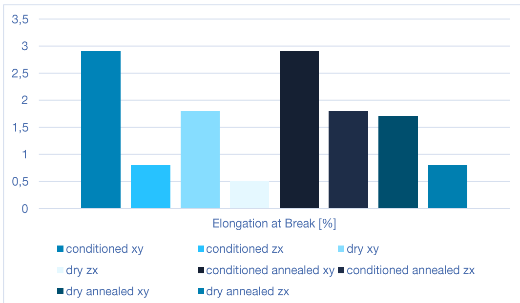
Elongation at Break comparison Ultrafuse® PAHT CF15 conditioned, dry and annealed
