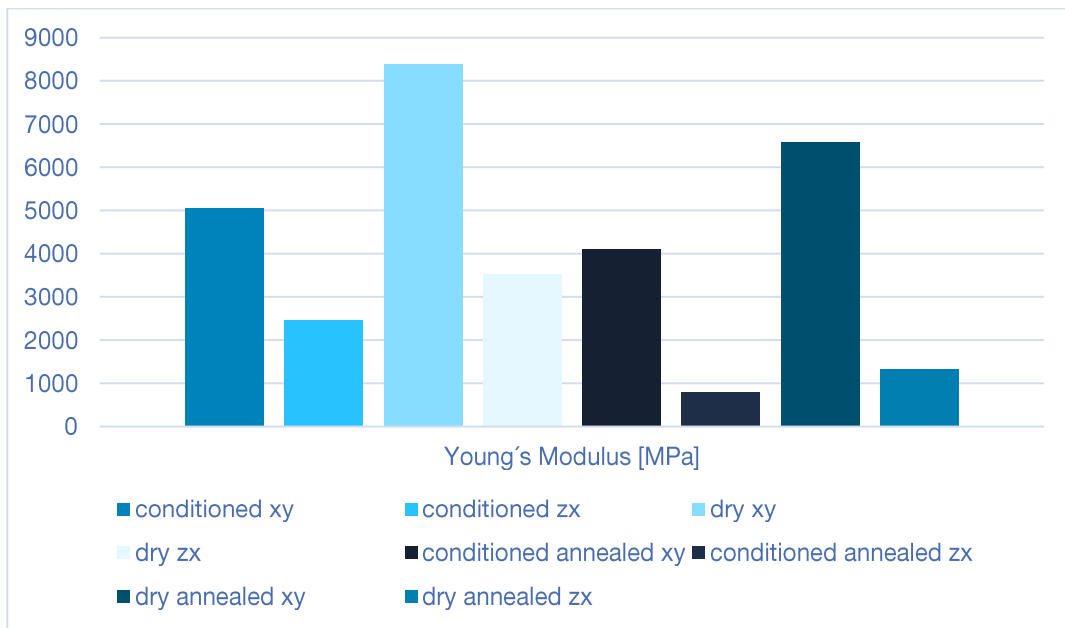
Young's Modulus comparison Ultrafuse® PAHT CF15 conditioned, dry and annealed
