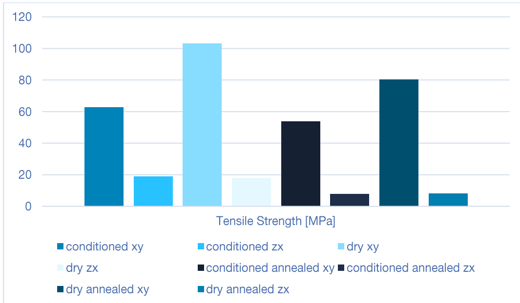
Tensile strength comparison Ultrafuse® PAHT CF15 conditioned, dry and annealed
